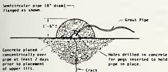
Fig. 3.8—Crack arrest method of crack repair
